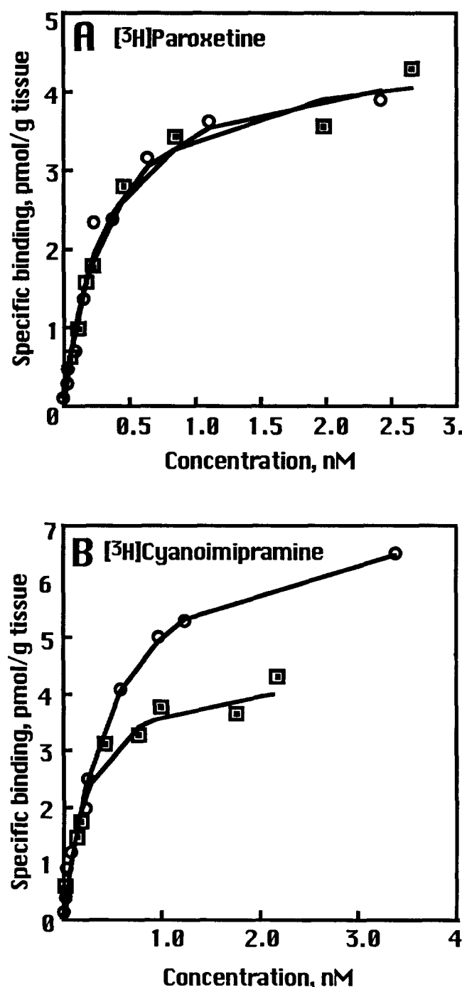
Figure 1. Saturation curves for [ ^3 H]paroxetine (A) and [ ^3 H]CN-IMI (B) binding to membrane preparations of the human putamen. Nonspecific binding was defined using 100 \mu mol/L desipramine or 150 \mu mol/L 5-HT. The binding conditions were as described in the Methods section. Nonspecific binding with: ○ 100 \mu M desipramine; ■ 150 \mu M 5-HT.
