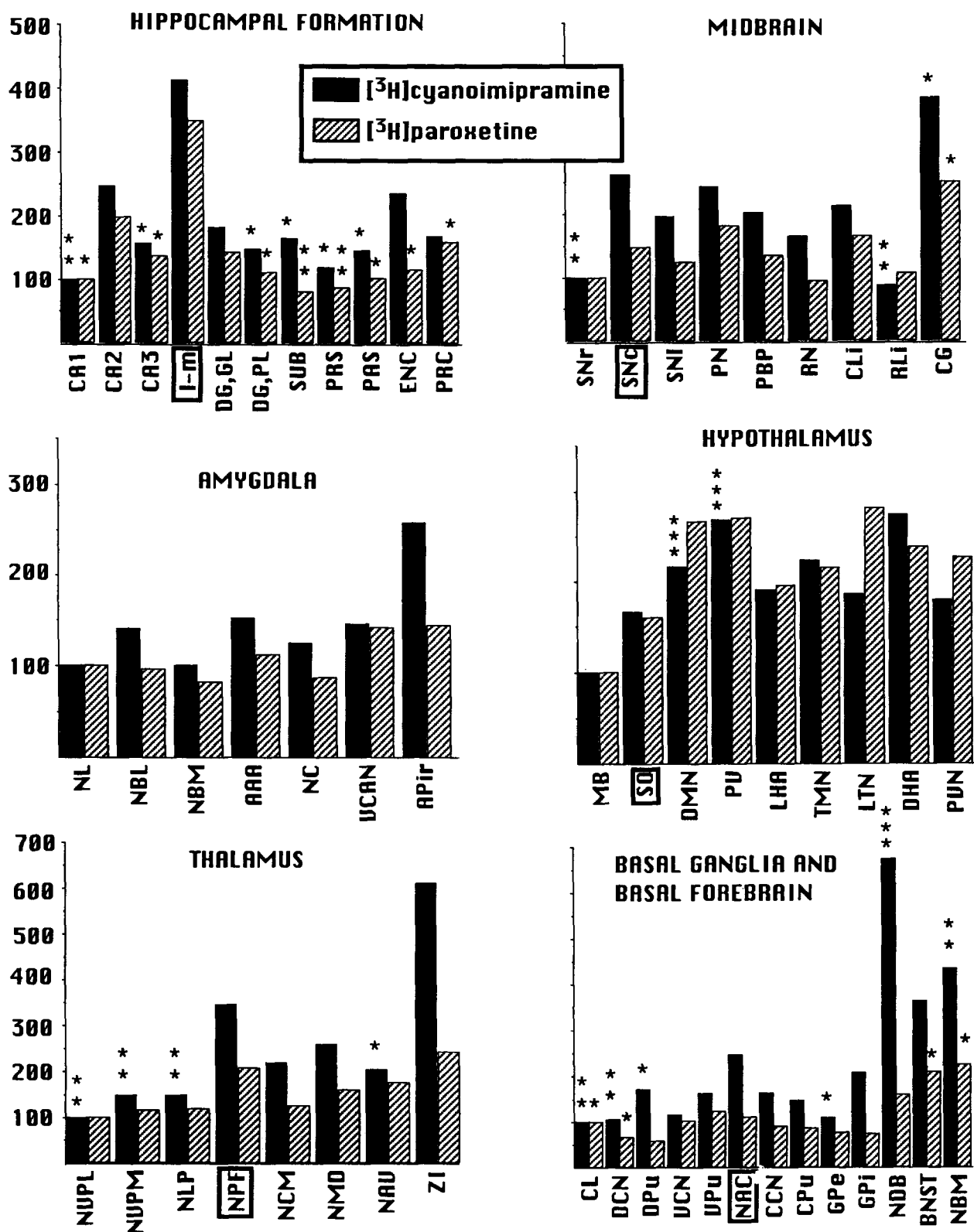
Figure 5. Relative binding profiles for [ 3 H]paroxetine and [ 3 H]CN-IMI in various brain regions. The values expressed as percentage of the binding in the regions with the lowest binding for [ 3 H]CN-IMI in each subdivision adjusted to 100% ( first bars on each graph ): CA1 field in the hippocampal formation, SNr in the midbrain, NL in the amygdala, MB in the hypothalamus, NVPL in the thalamus, and Cl in the basal ganglia. The data were analyzed by one-way ANOVA with brain region as main factor. The main effect was significant for [ 3 H]CN-IMI binding ( F = 61.9 (5, 264), p = .0001 ) as well as for [ 3 H]paroxetine binding ( F = 18.3 (5, 237), p = .0001 ). Asterisks denote statistically significant differences with * p < 0.05 , ** p < .01 , and *** p < .001 .
